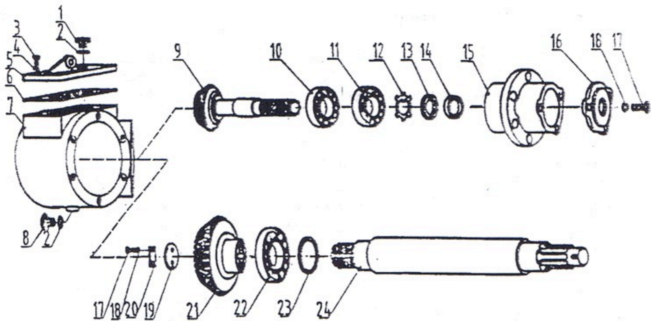
Power Shaft Assembly
